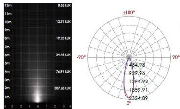
Lux distance curve
